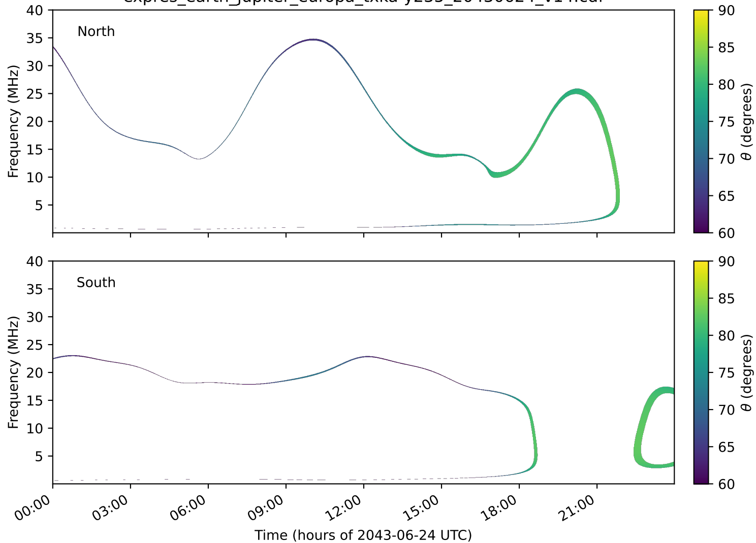
expres_earth_jupiter_europa_txka-y235_20430624_v14.cdf
