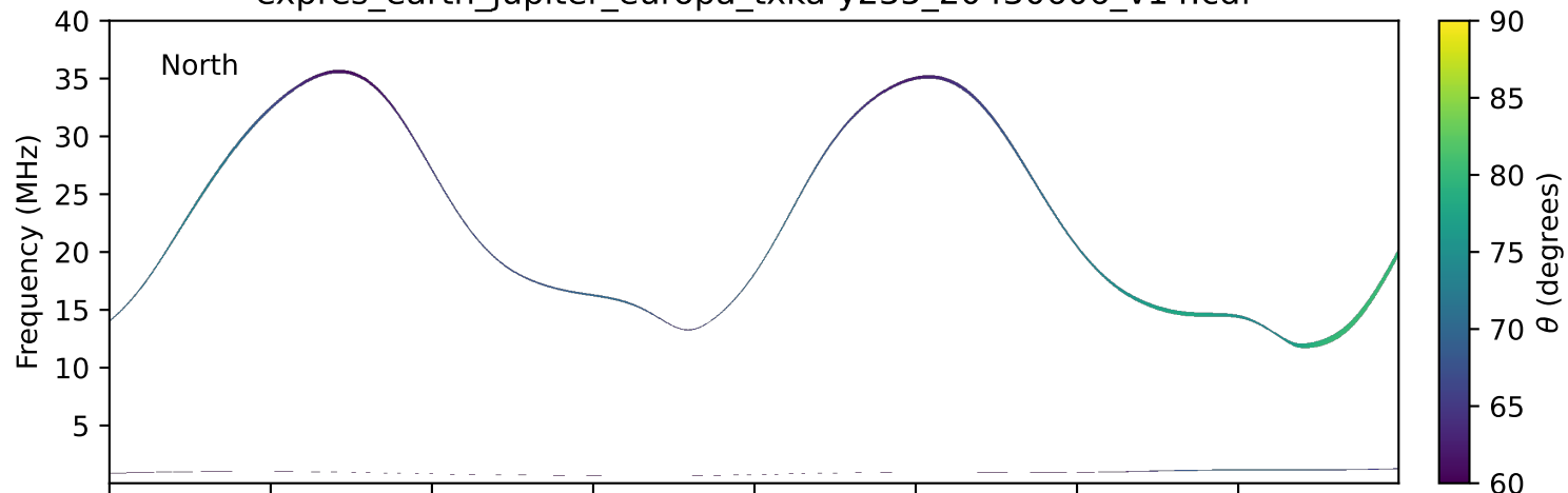
expres_earth_jupiter_europa_txka-y235_20430606_v14.cdf
