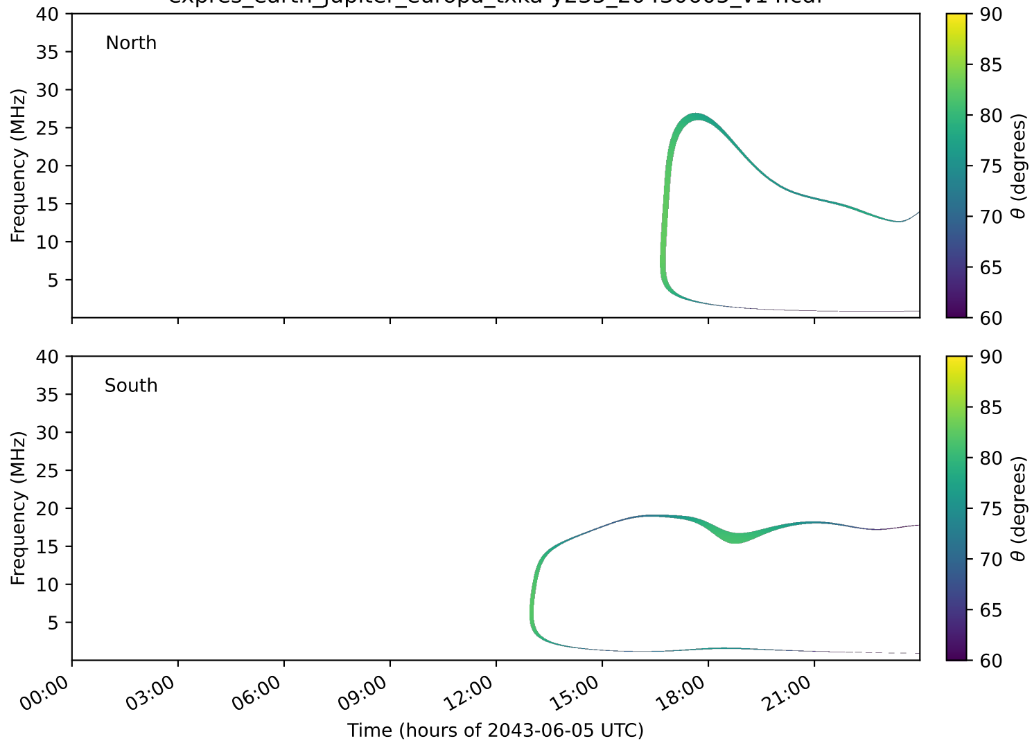
expres_earth_jupiter_europa_txka-y235_20430605_v14.cdf
