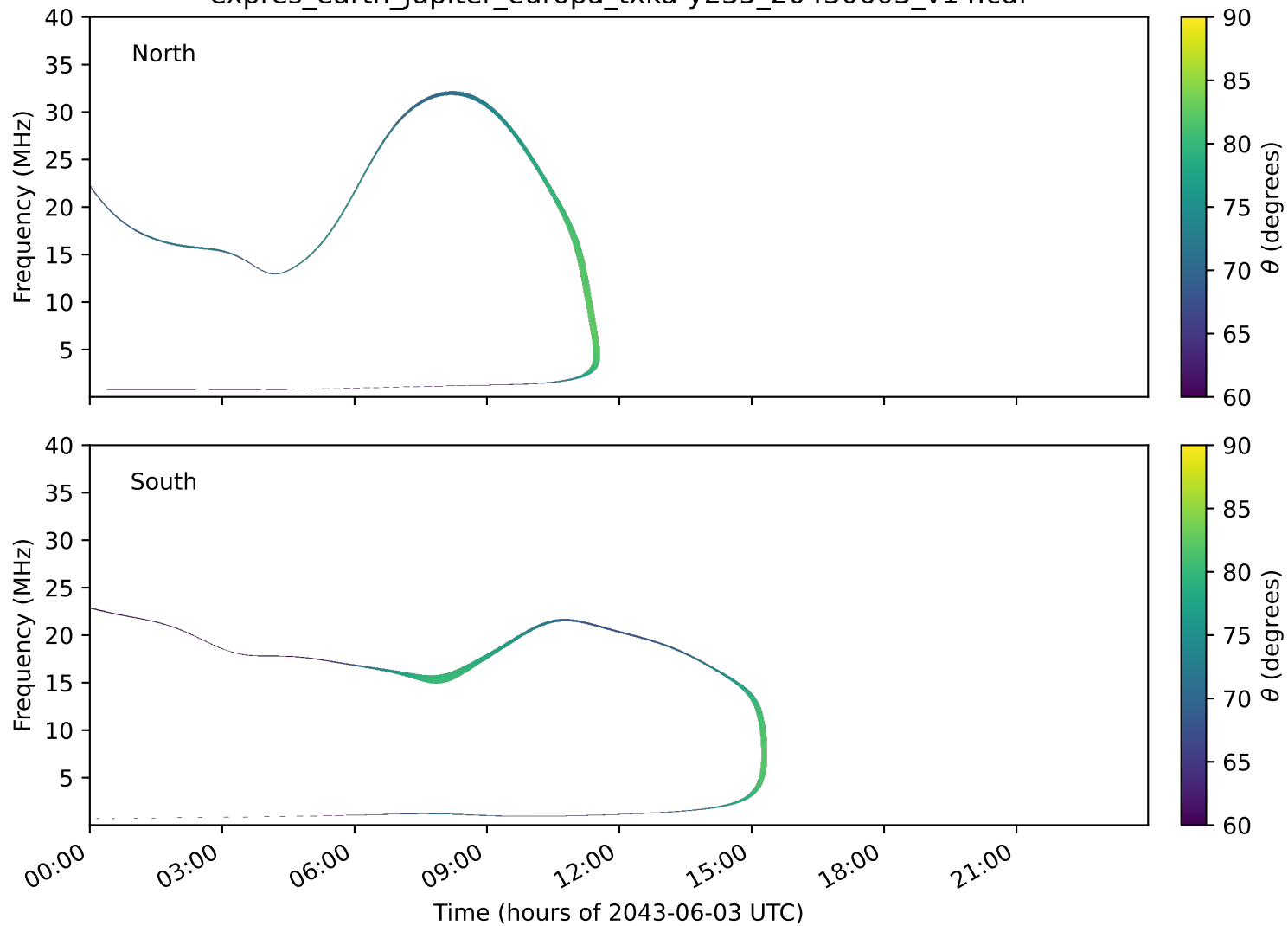
expres_earth_jupiter_europa_txka-y235_20430603_v14.cdf
