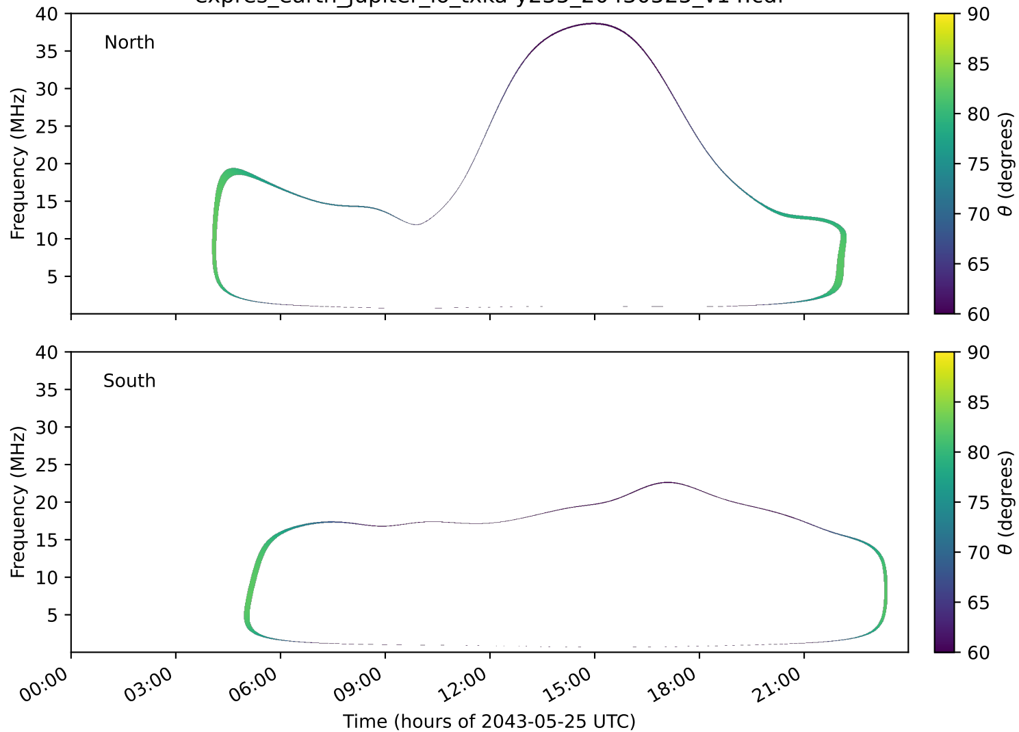
expres_earth_jupiter_io_txka-y235_20430525_v14.cdf
