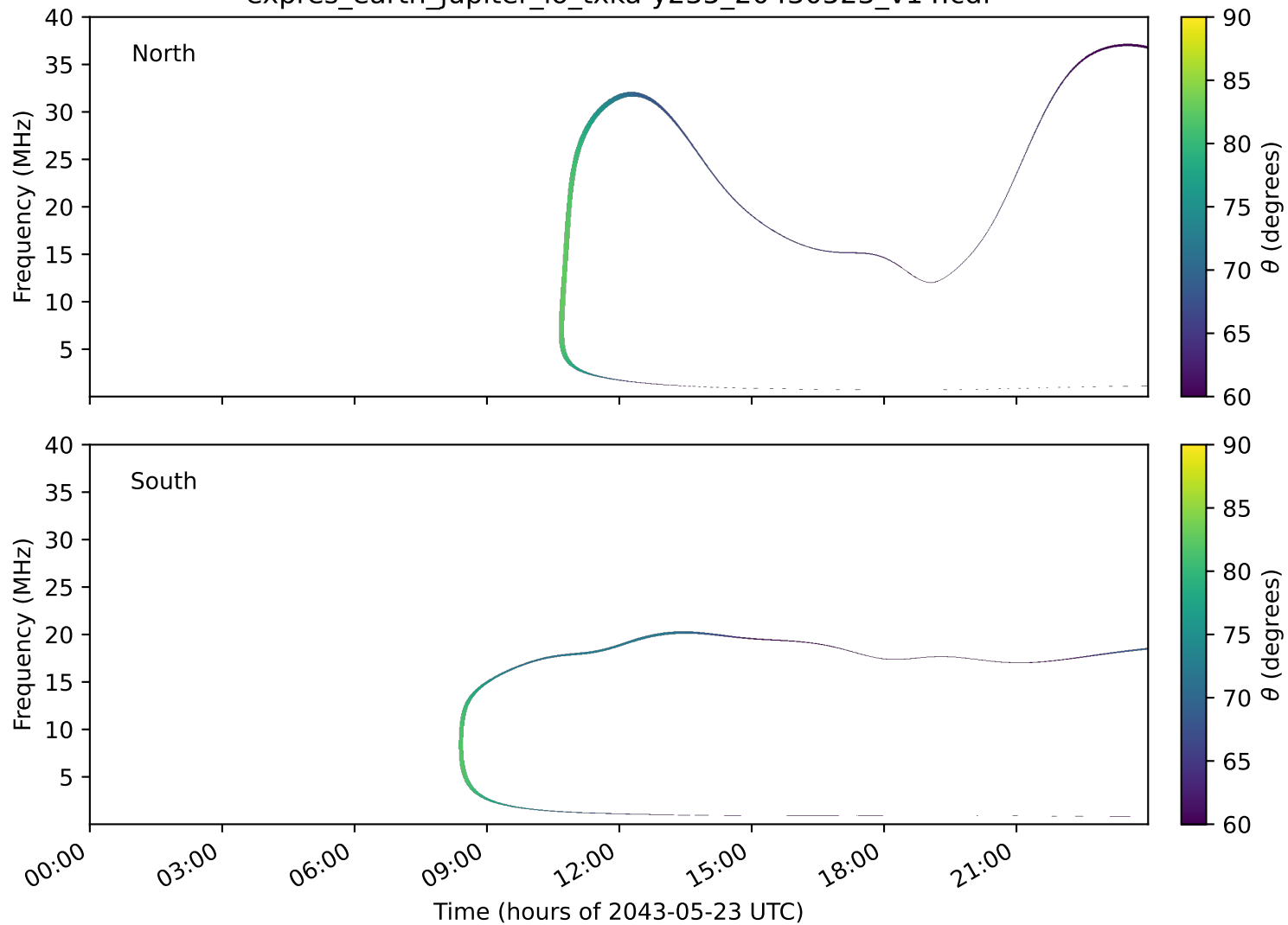
expres_earth_jupiter_io_txka-y235_20430523_v14.cdf
