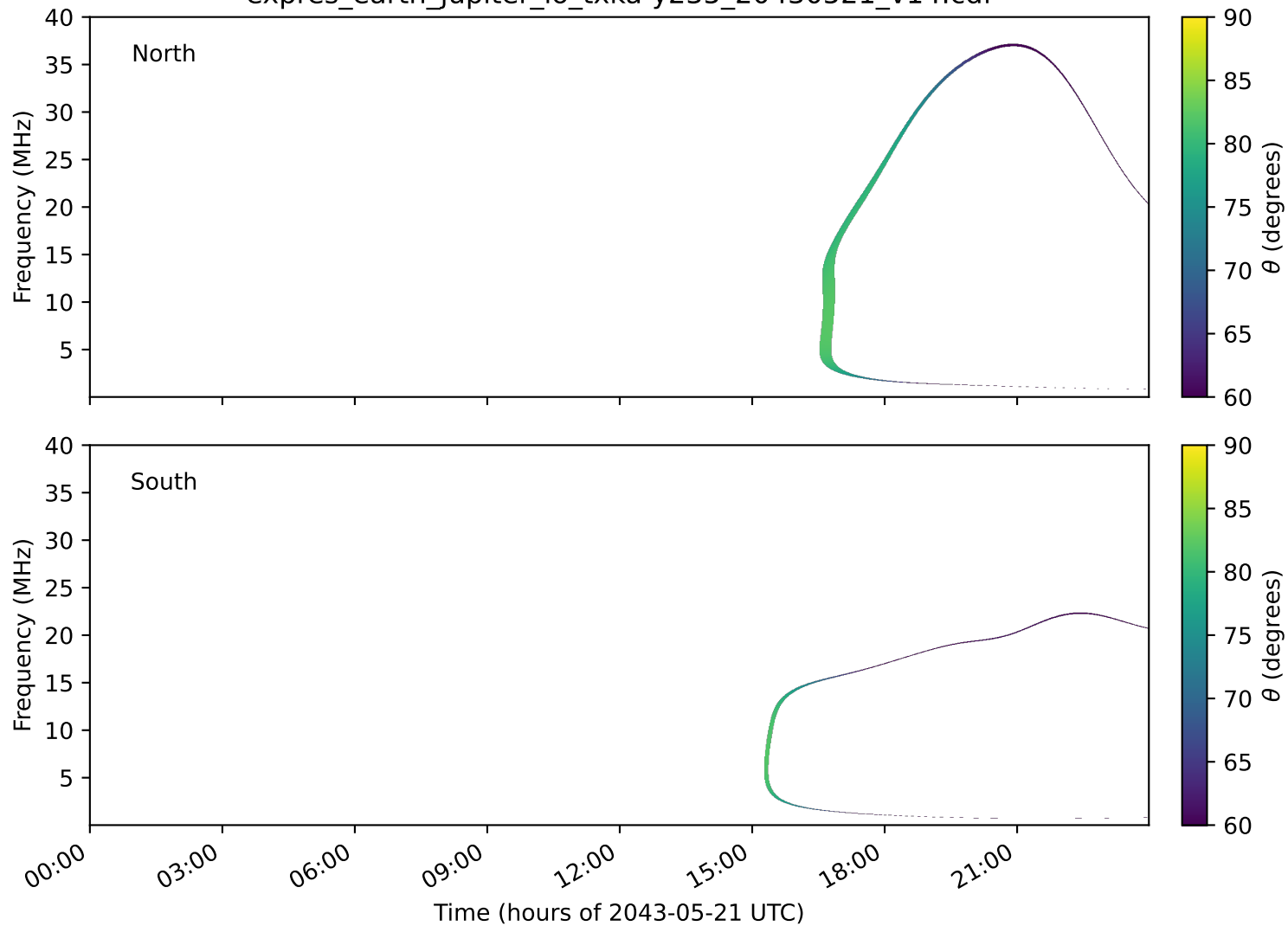
expres_earth_jupiter_io_txka-y235_20430521_v14.cdf
