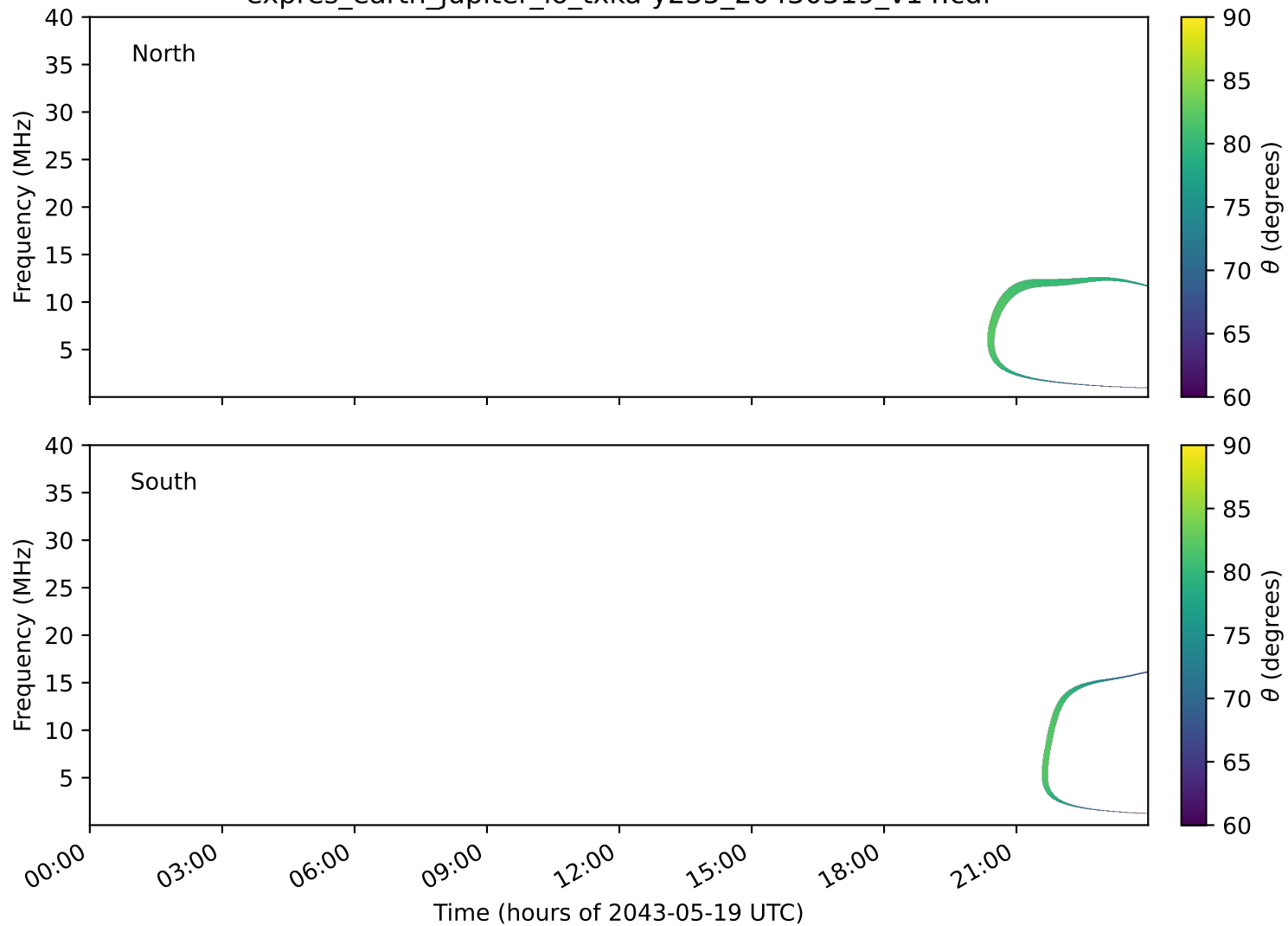
expres_earth_jupiter_io_txka-y235_20430519_v14.cdf
