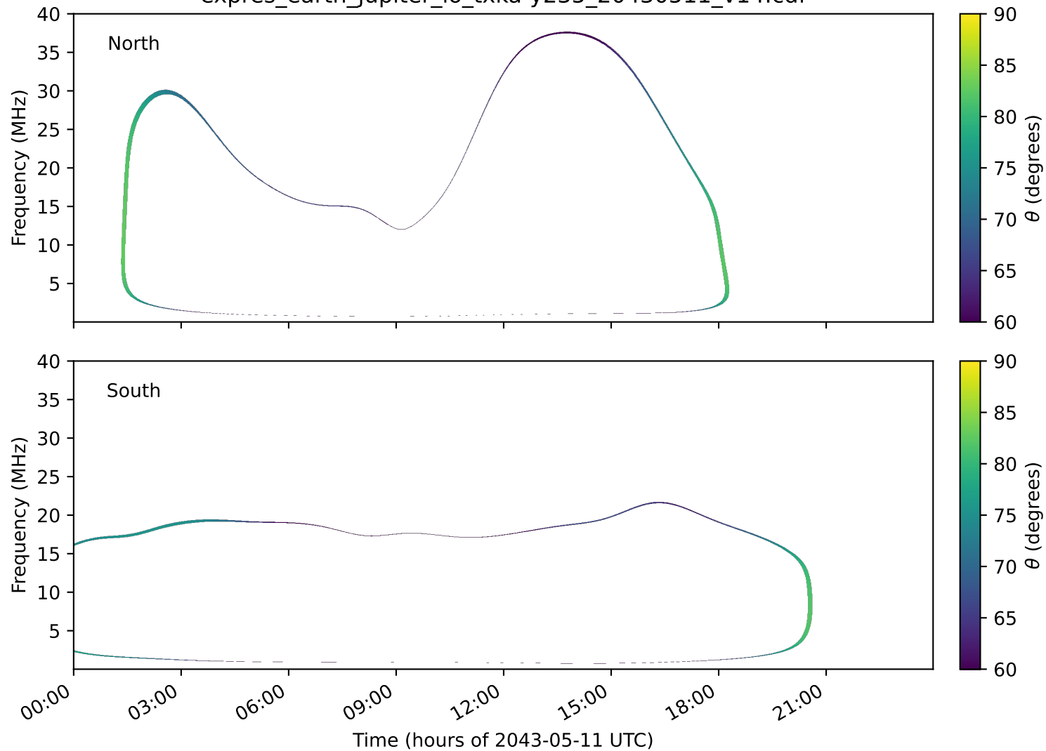
expres_earth_jupiter_io_txka-y235_20430511_v14.cdf
