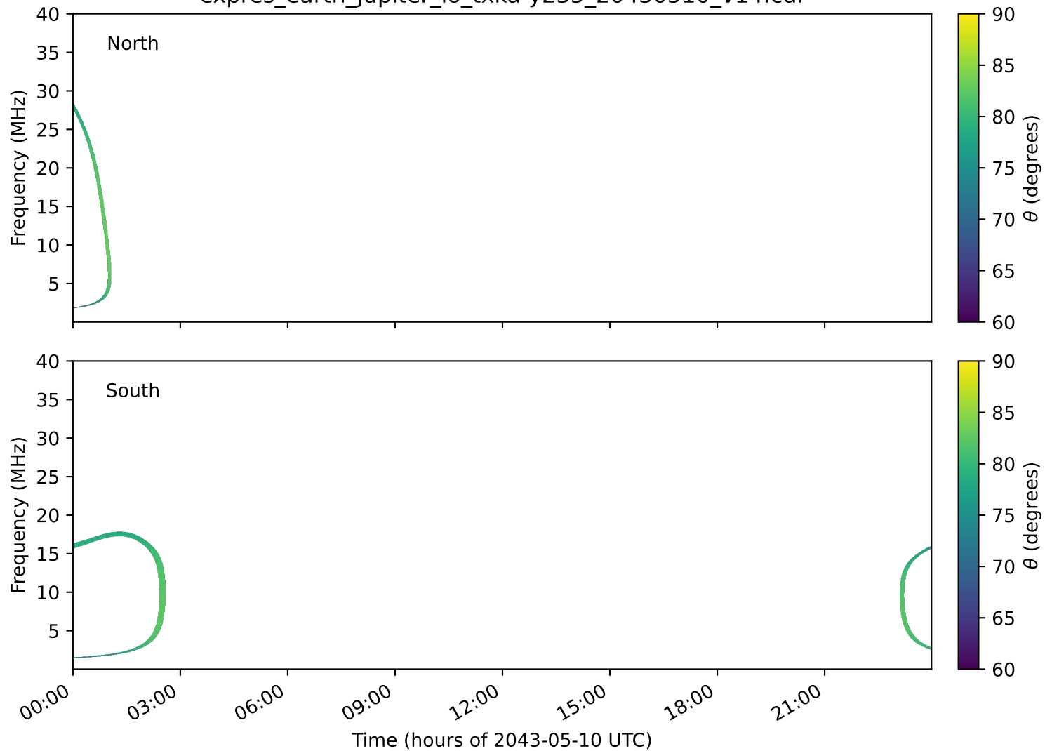
expres_earth_jupiter_io_txka-y235_20430510_v14.cdf
