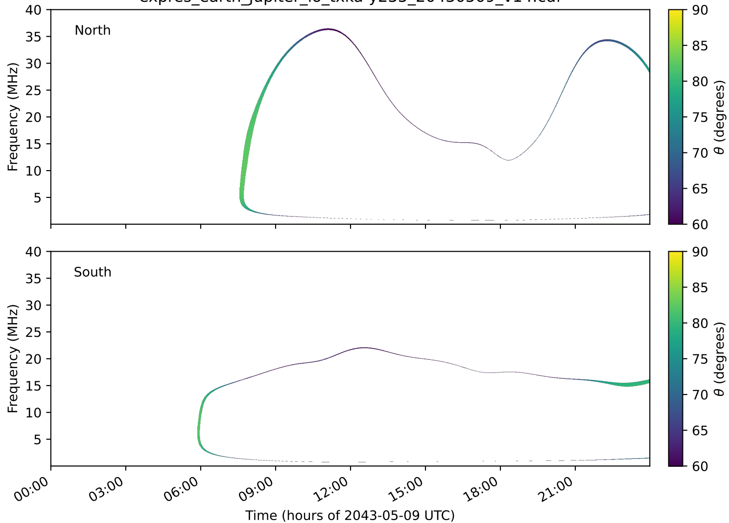
expres_earth_jupiter_io_txka-y235_20430509_v14.cdf
