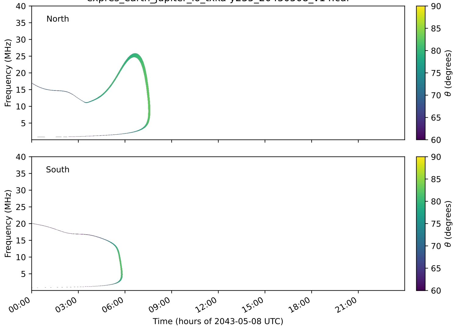
expres_earth_jupiter_io_txka-y235_20430508_v14.cdf
