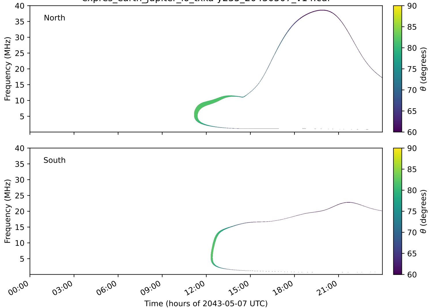
expres_earth_jupiter_io_txka-y235_20430507_v14.cdf
