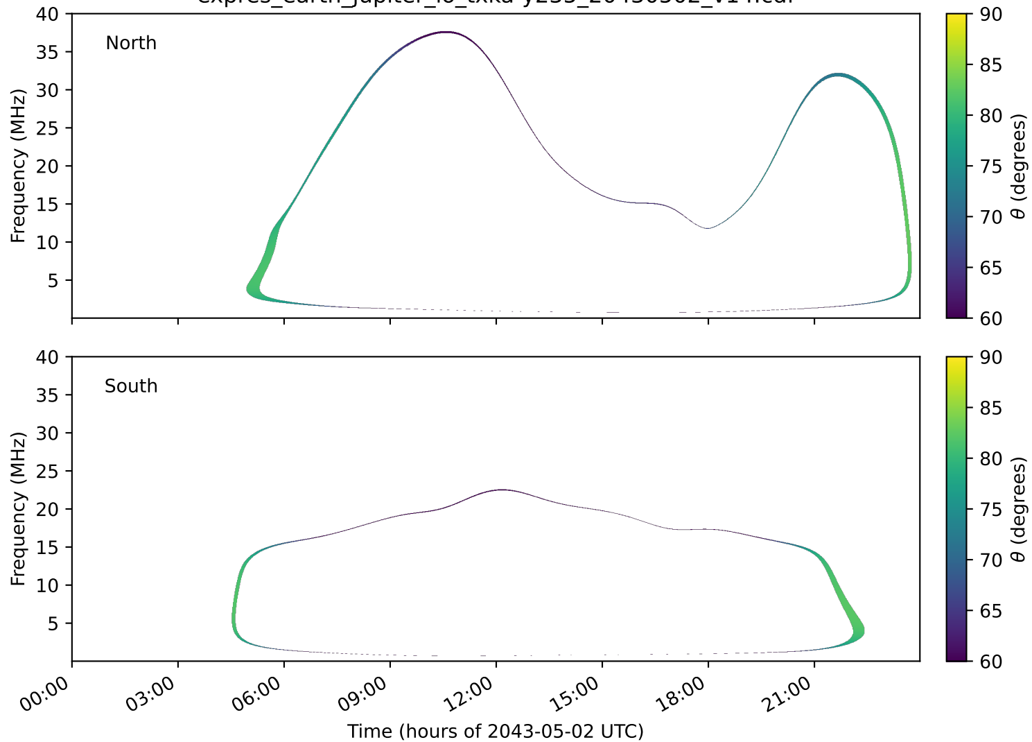
expres_earth_jupiter_io_txka-y235_20430502_v14.cdf
