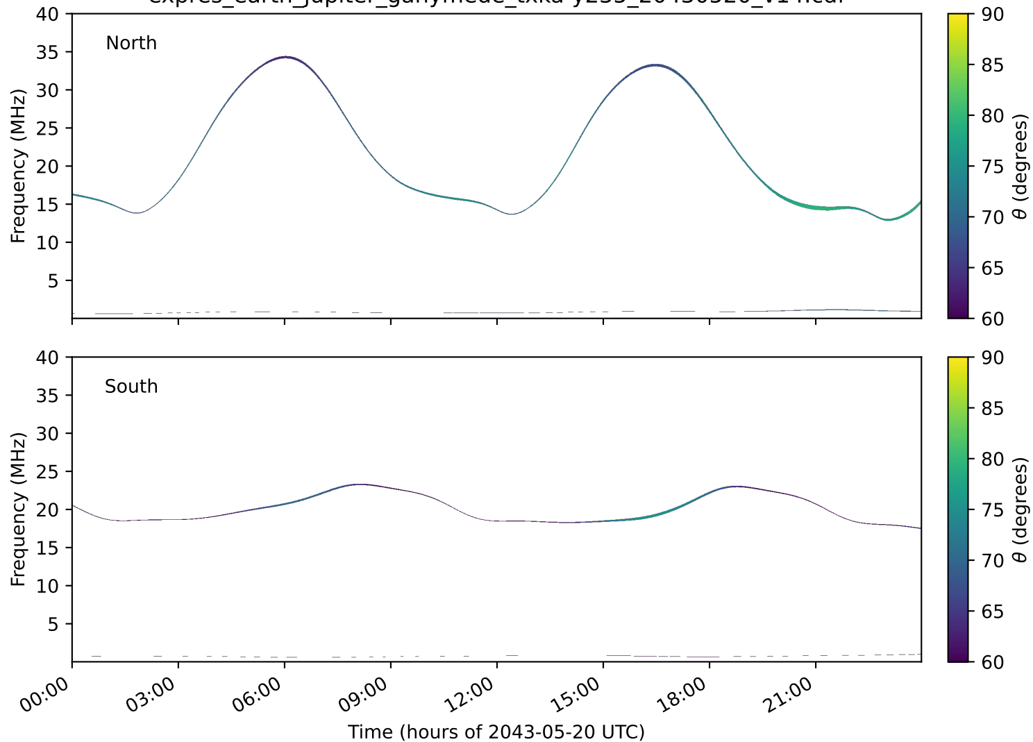
expres_earth_jupiter_ganymede_txka-y235_20430520_v14.cdf
