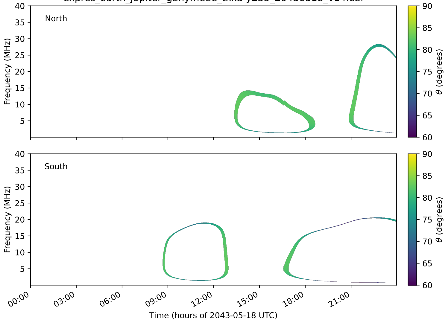
expres_earth_jupiter_ganymede_txka-y235_20430518_v14.cdf
