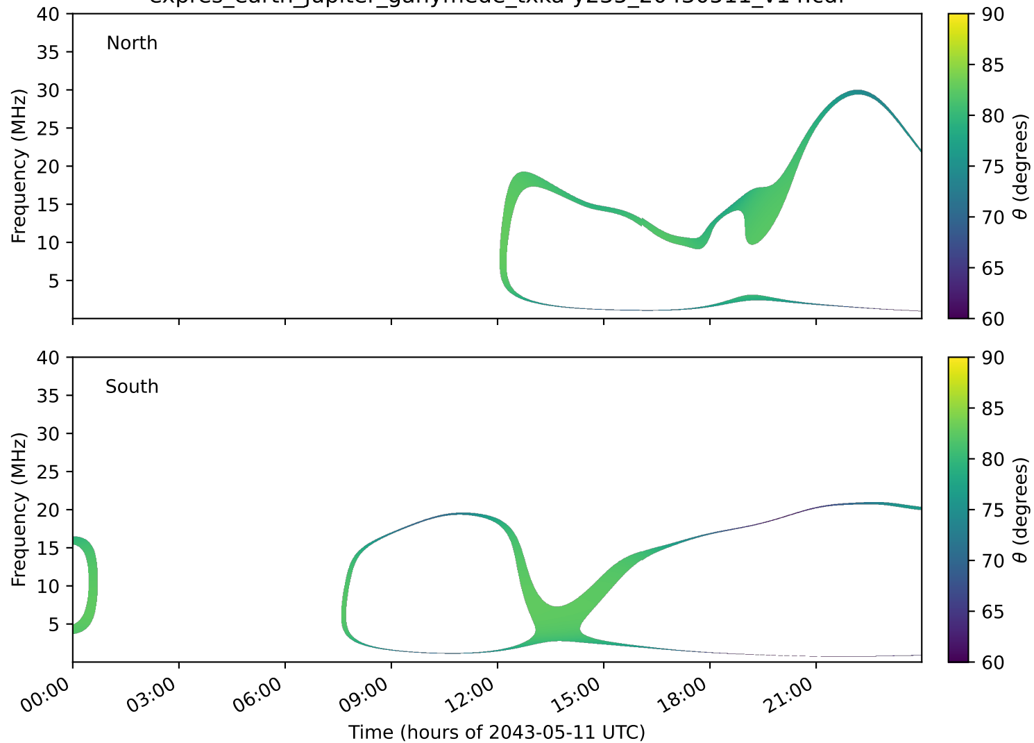
expres_earth_jupiter_ganymede_txka-y235_20430511_v14.cdf
