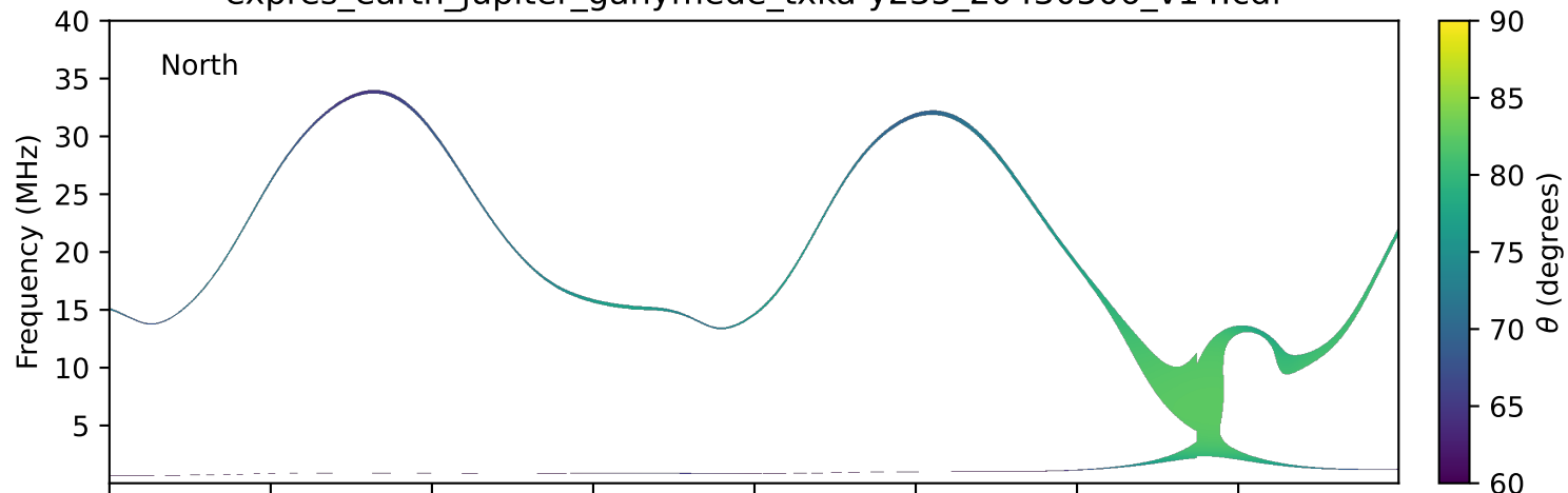
expres_earth_jupiter_ganymede_txka-y235_20430506_v14.cdf
