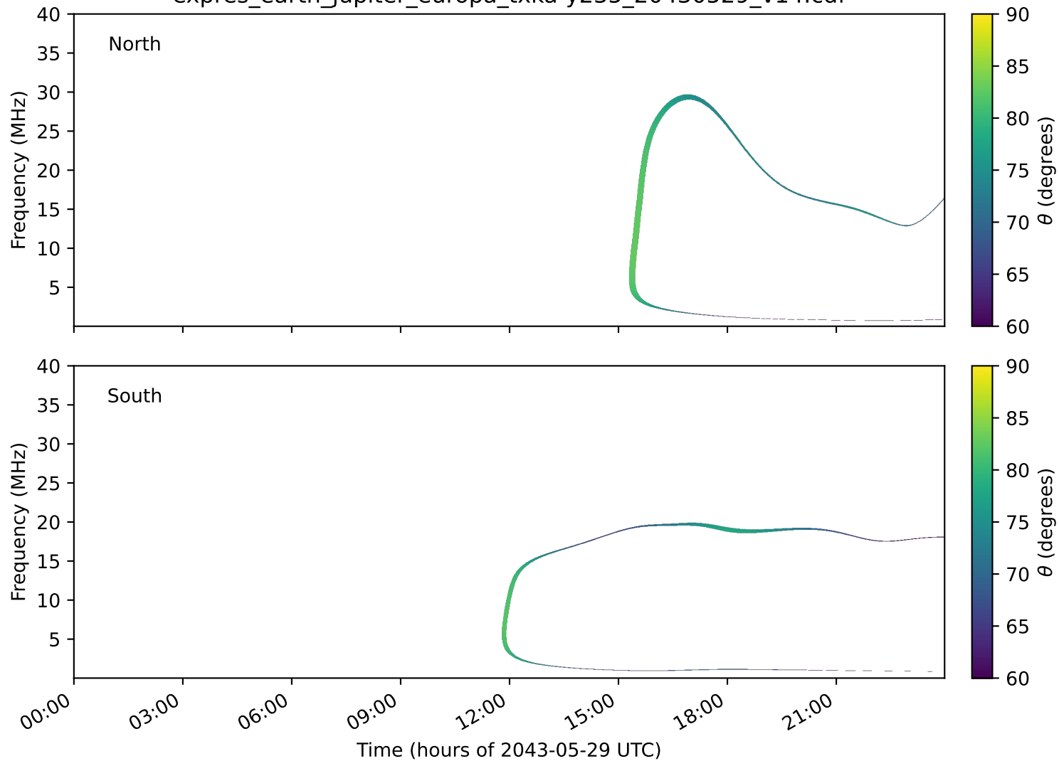
expres_earth_jupiter_europa_txka-y235_20430529_v14.cdf
