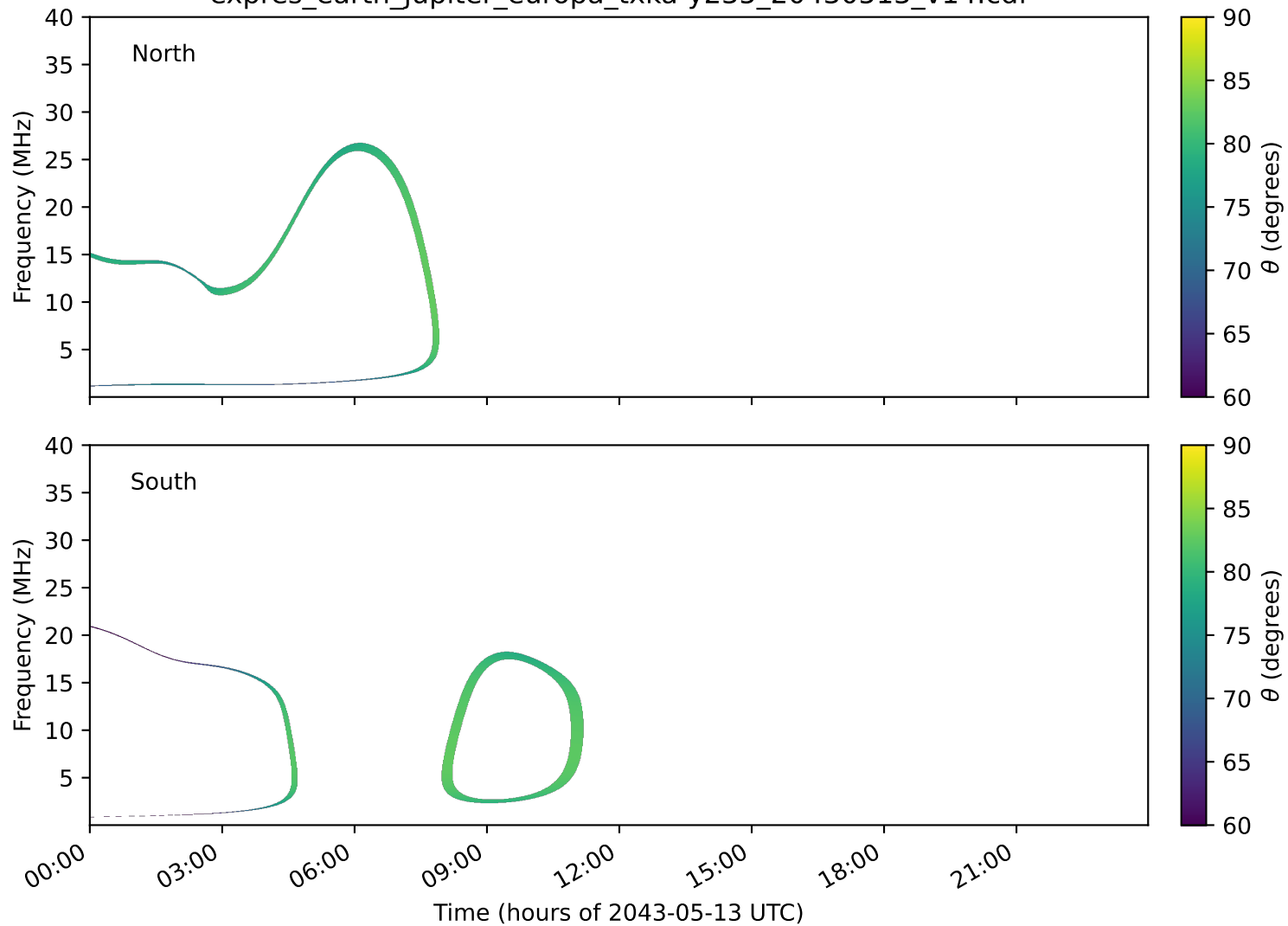
expres_earth_jupiter_europa_txka-y235_20430513_v14.cdf
