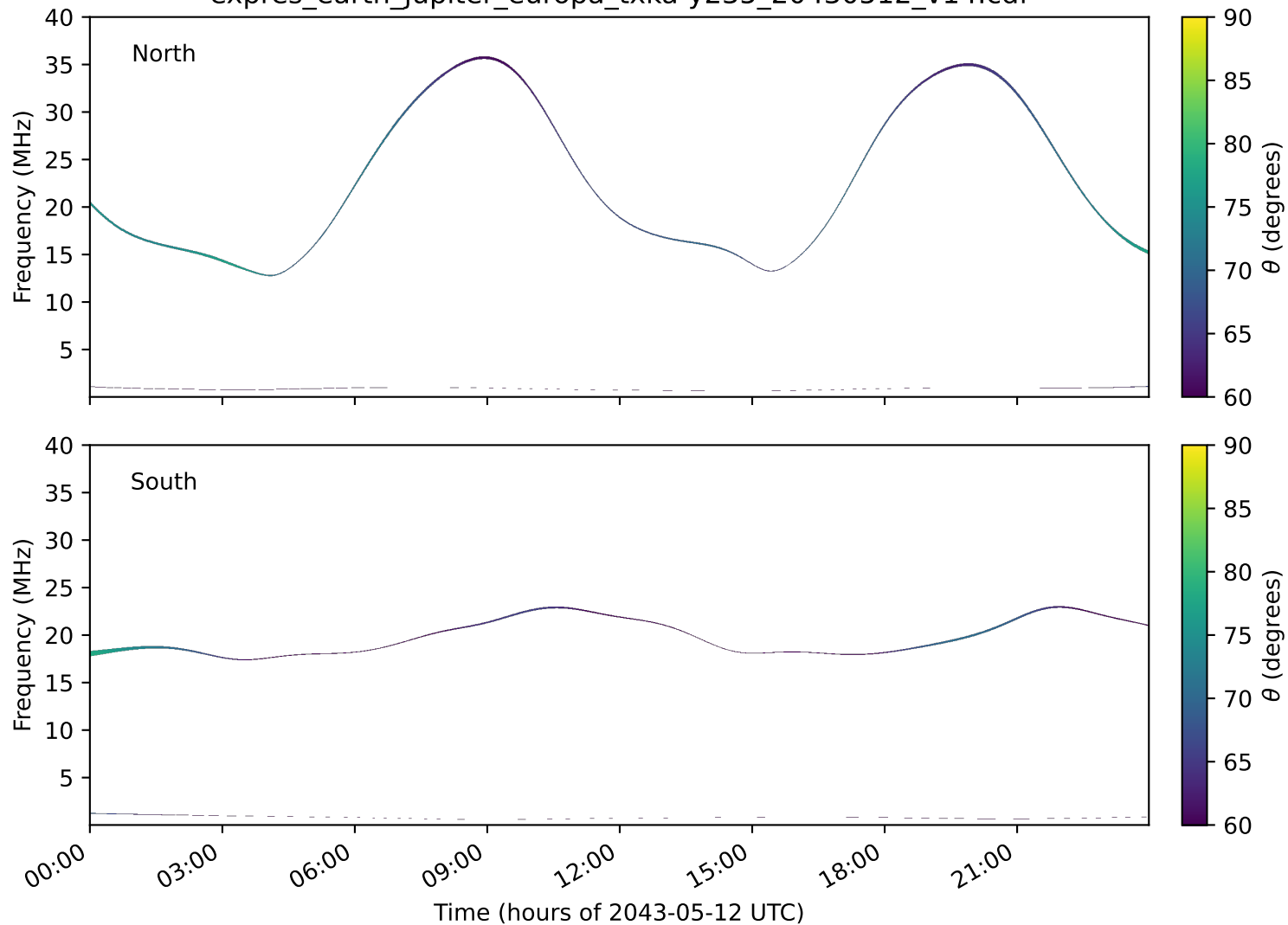
expres_earth_jupiter_europa_txka-y235_20430512_v14.cdf
