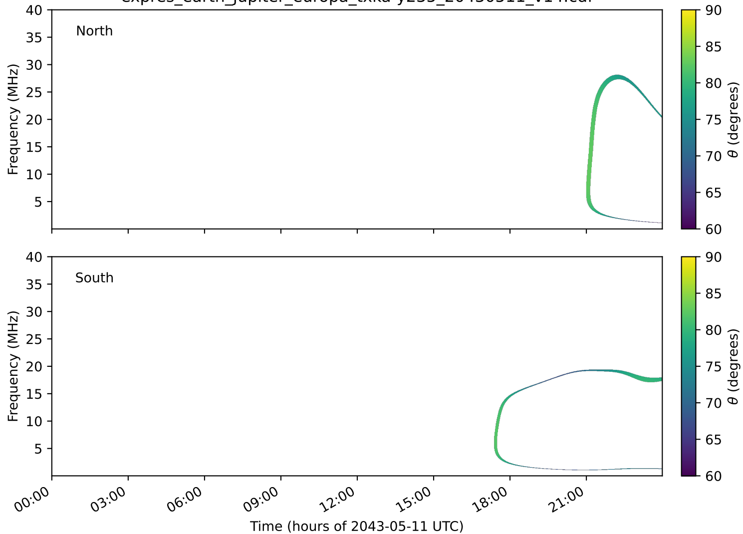
expres_earth_jupiter_europa_txka-y235_20430511_v14.cdf
