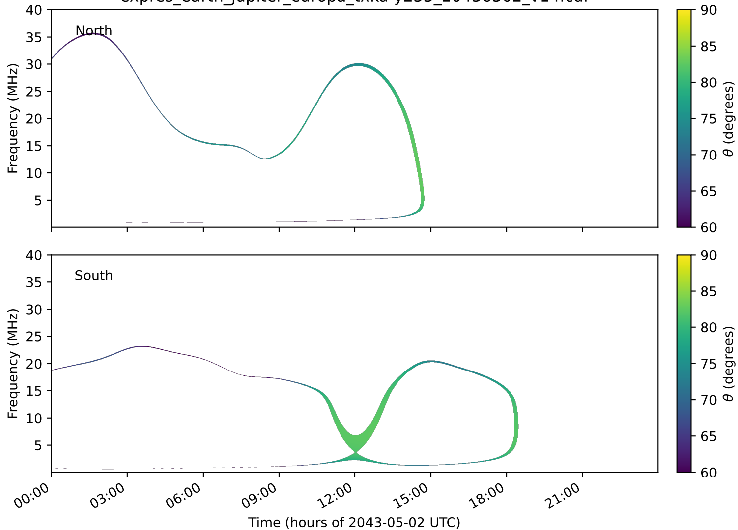
expres_earth_jupiter_europa_txka-y235_20430502_v14.cdf
