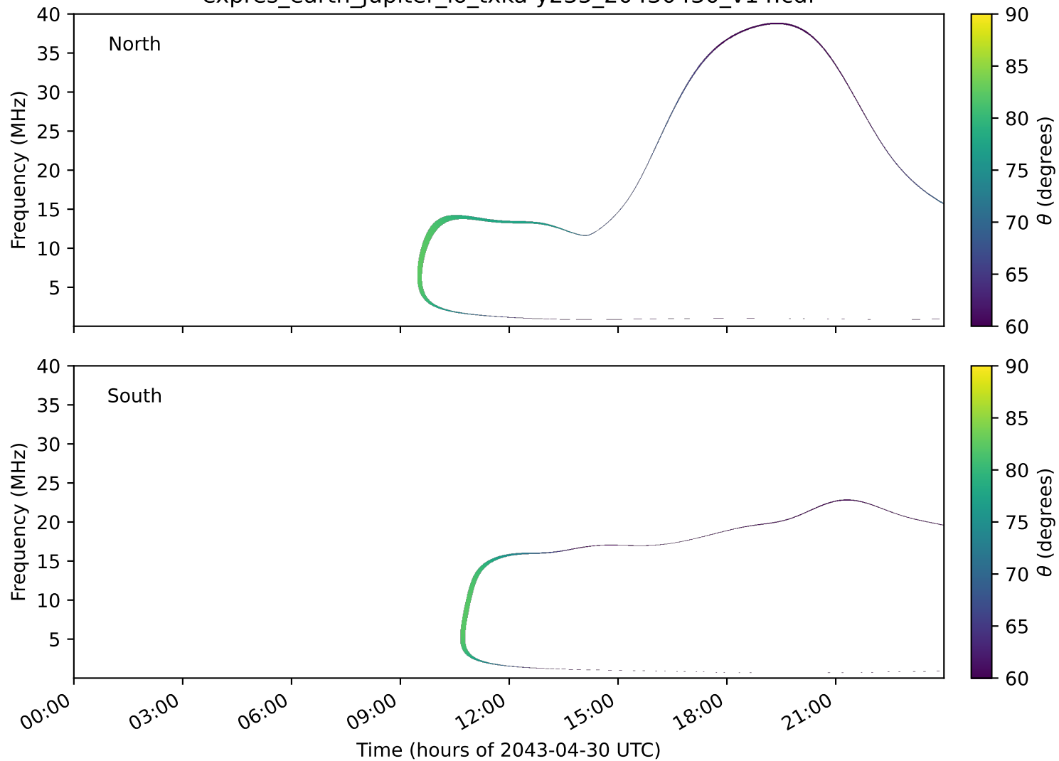
expres_earth_jupiter_io_txka-y235_20430430_v14.cdf
