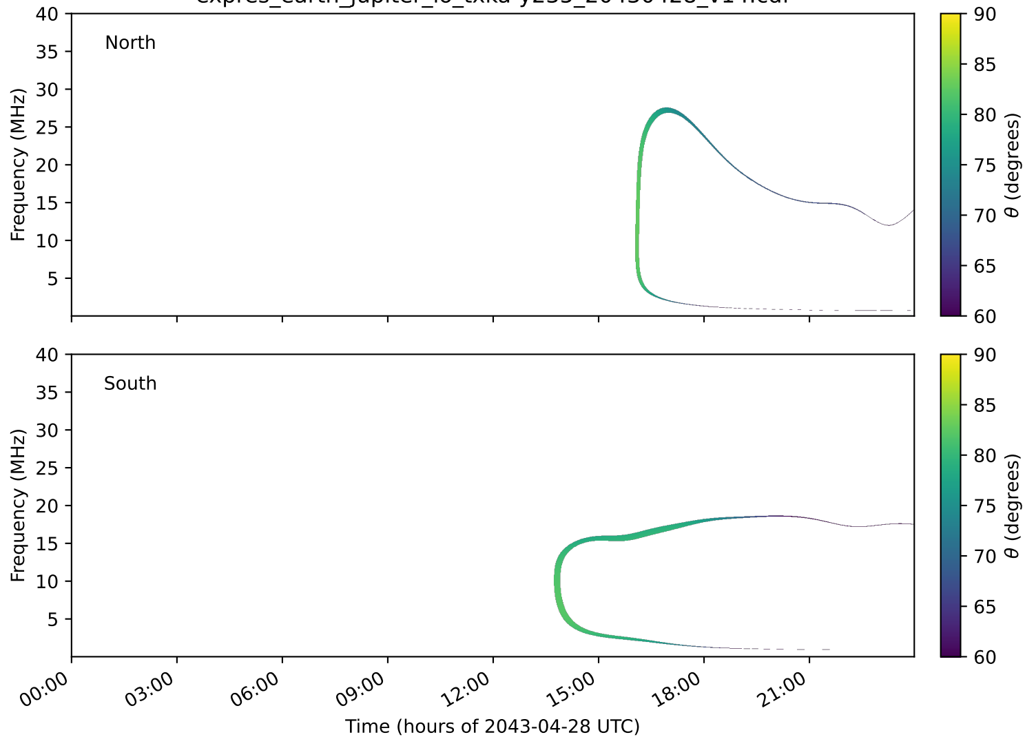
expres_earth_jupiter_io_txka-y235_20430428_v14.cdf
