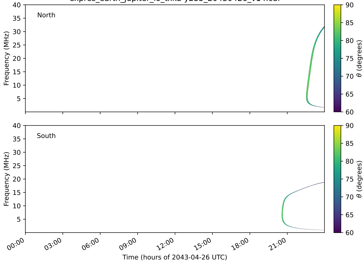
expres_earth_jupiter_io_txka-y235_20430426_v14.cdf
