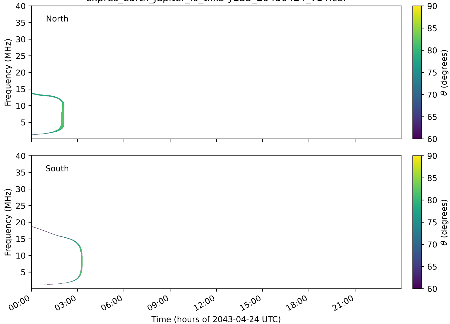
expres_earth_jupiter_io_txka-y235_20430424_v14.cdf
