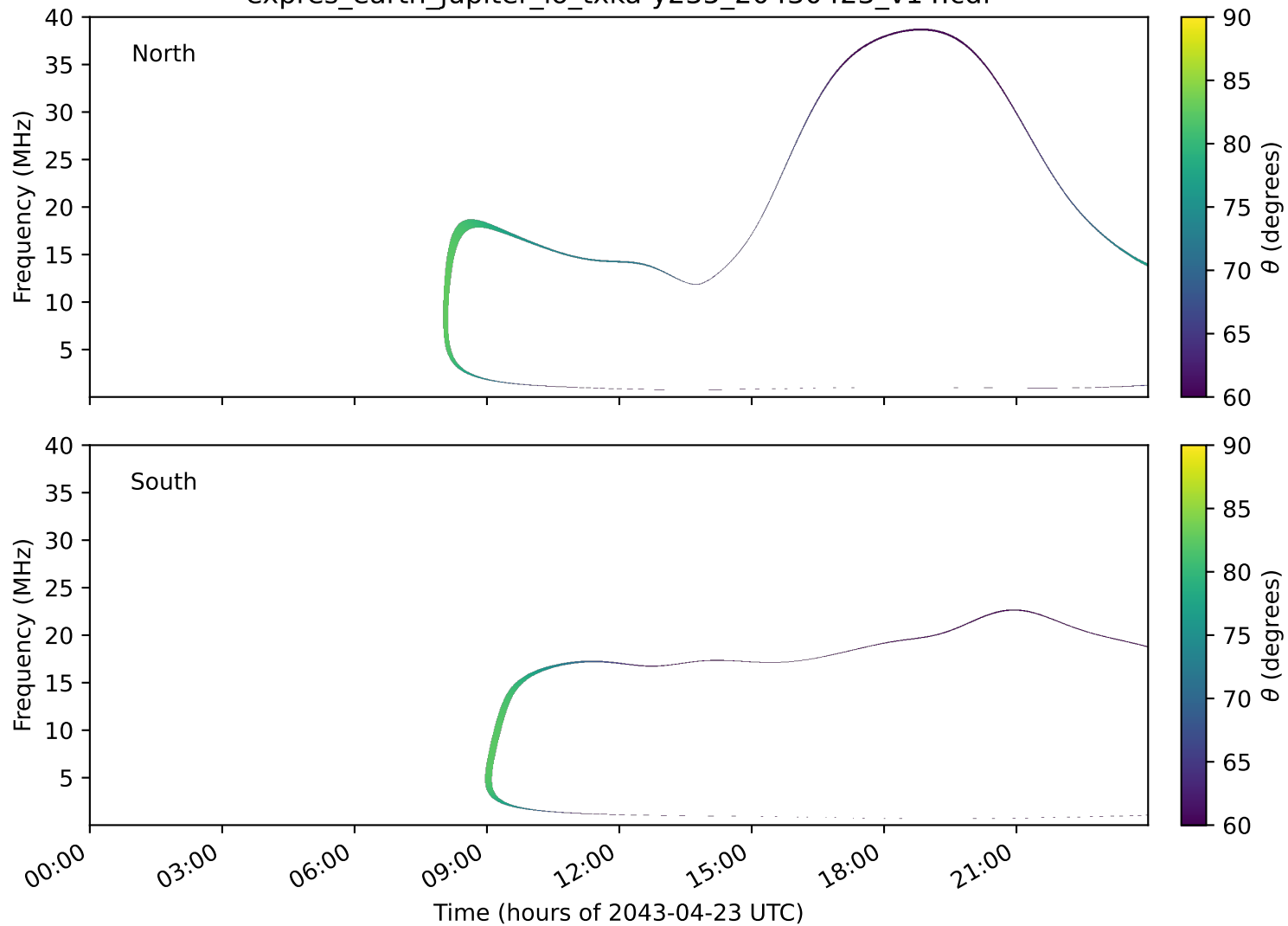
expres_earth_jupiter_io_txka-y235_20430423_v14.cdf
