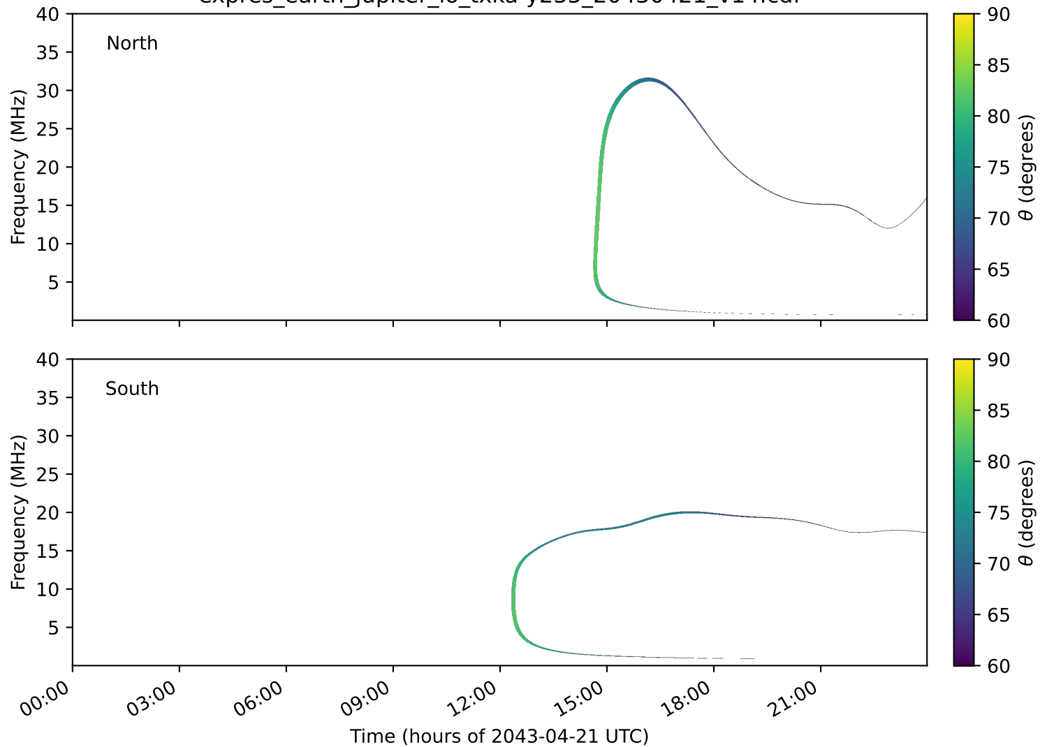
expres_earth_jupiter_io_txka-y235_20430421_v14.cdf
