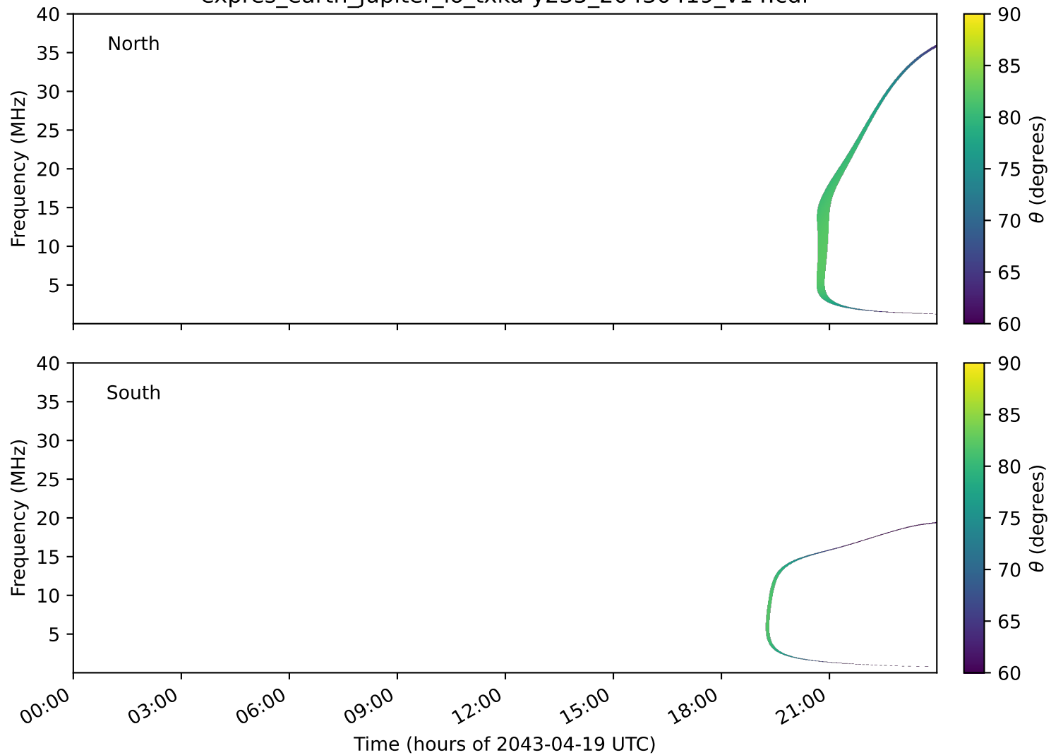
expres_earth_jupiter_io_txka-y235_20430419_v14.cdf
