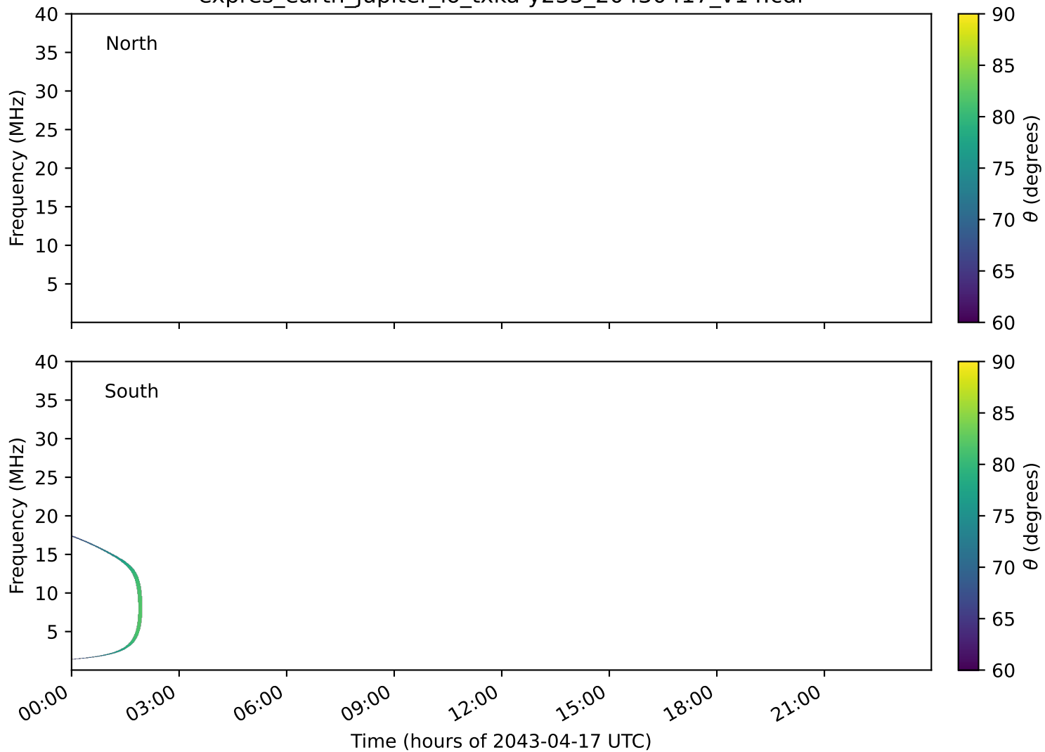
expres_earth_jupiter_io_txka-y235_20430417_v14.cdf
