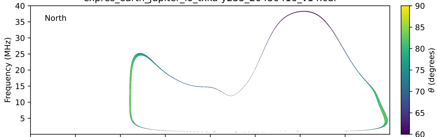
expres_earth_jupiter_io_txka-y235_20430416_v14.cdf
