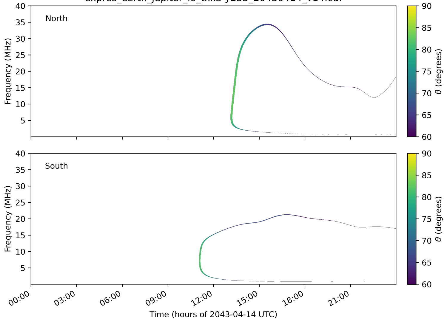
expres_earth_jupiter_io_txka-y235_20430414_v14.cdf
