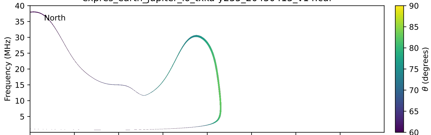
expres_earth_jupiter_io_txka-y235_20430413_v14.cdf
