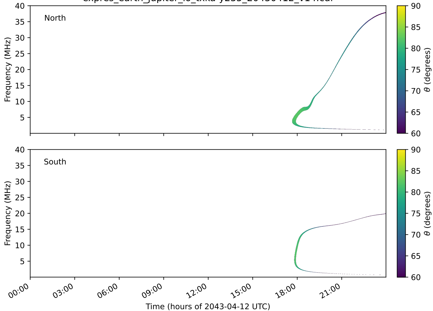
expres_earth_jupiter_io_txka-y235_20430412_v14.cdf
