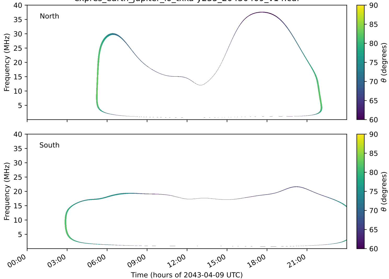
expres_earth_jupiter_io_txka-y235_20430409_v14.cdf
