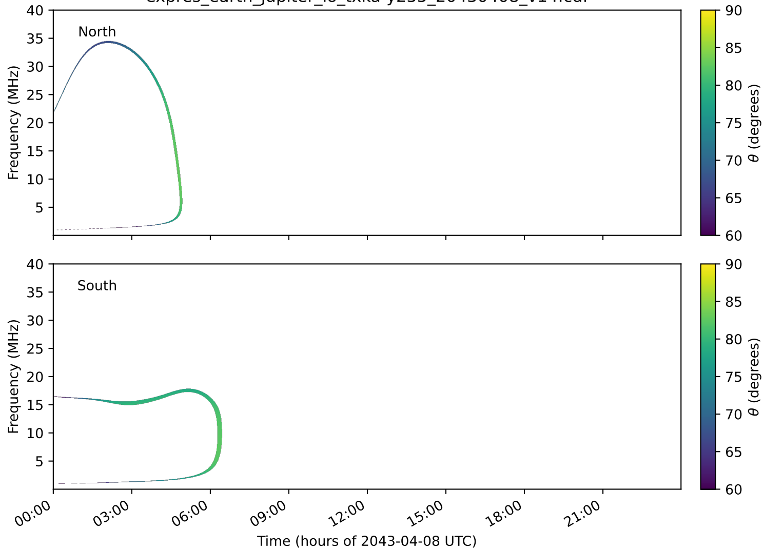
expres_earth_jupiter_io_txka-y235_20430408_v14.cdf
