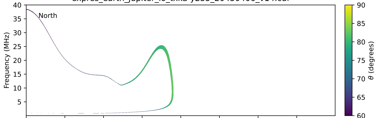
expres_earth_jupiter_io_txka-y235_20430406_v14.cdf
