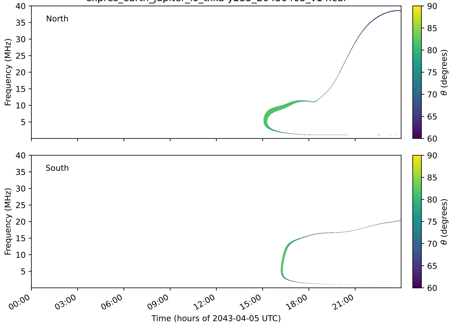
expres_earth_jupiter_io_txka-y235_20430405_v14.cdf
