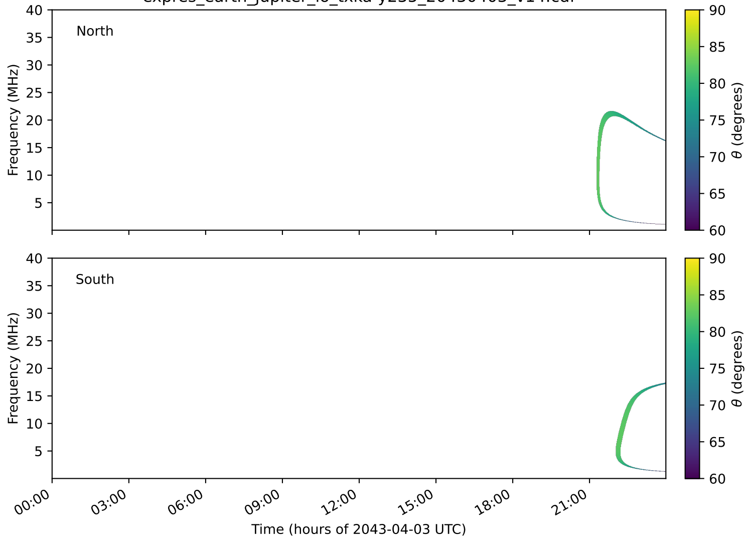
expres_earth_jupiter_io_txka-y235_20430403_v14.cdf
