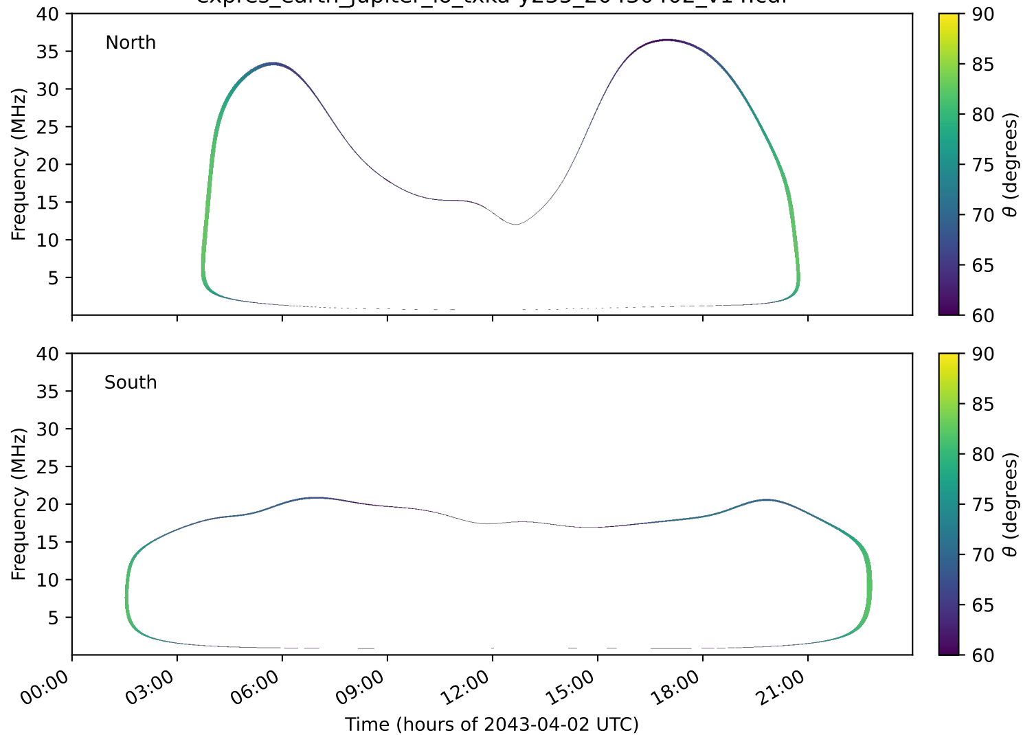
expres_earth_jupiter_io_txka-y235_20430402_v14.cdf
