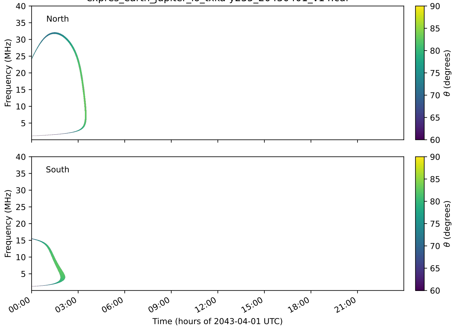
expres_earth_jupiter_io_txka-y235_20430401_v14.cdf
