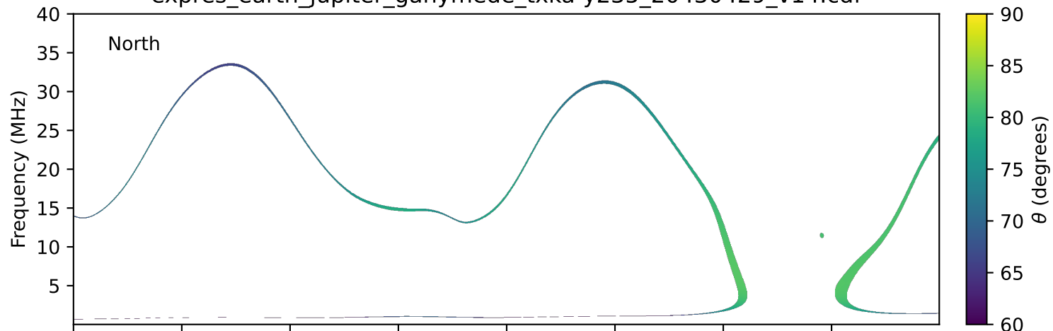
expres_earth_jupiter_ganymede_txka-y235_20430429_v14.cdf
