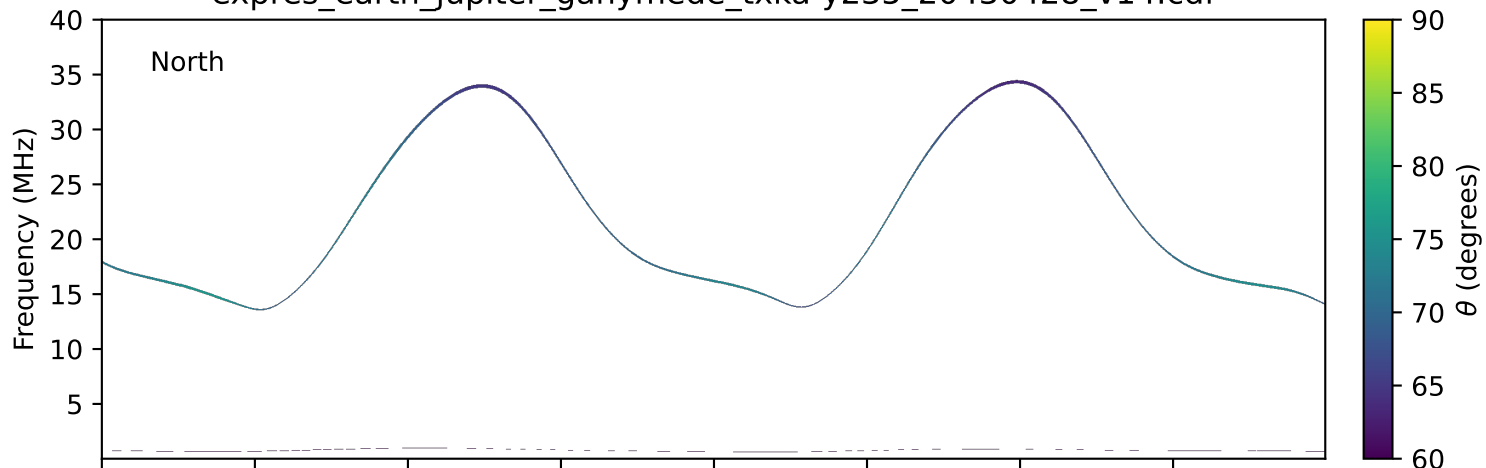
expres_earth_jupiter_ganymede_txka-y235_20430428_v14.cdf
