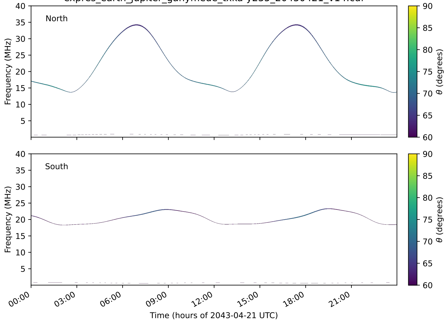
expres_earth_jupiter_ganymede_txka-y235_20430421_v14.cdf
