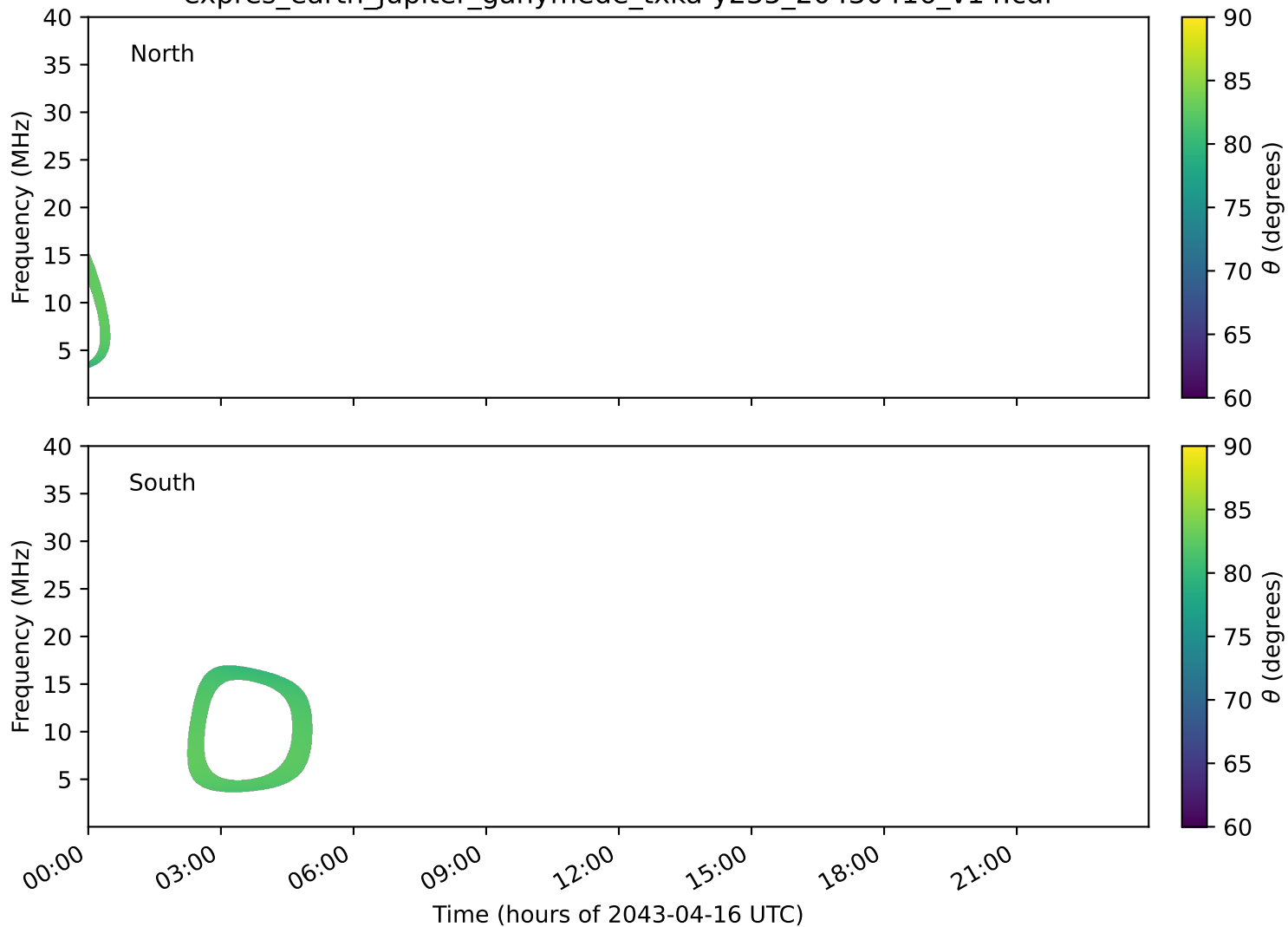
expres_earth_jupiter_ganymede_txka-y235_20430416_v14.cdf
