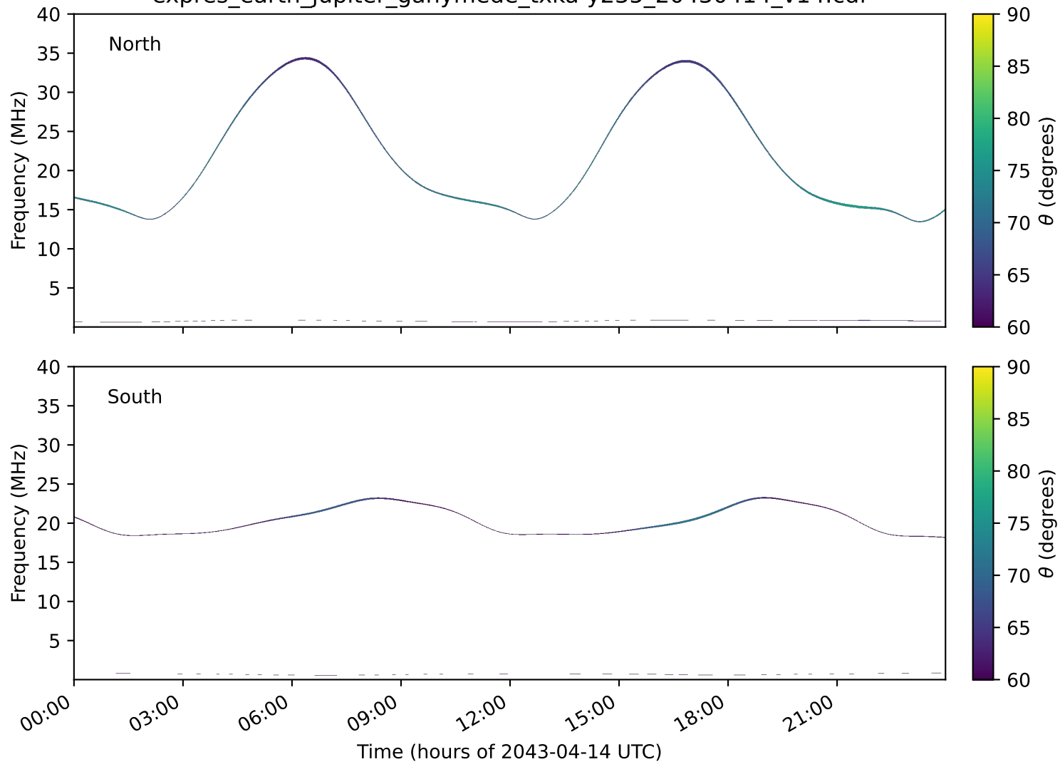
expres_earth_jupiter_ganymede_txka-y235_20430414_v14.cdf
