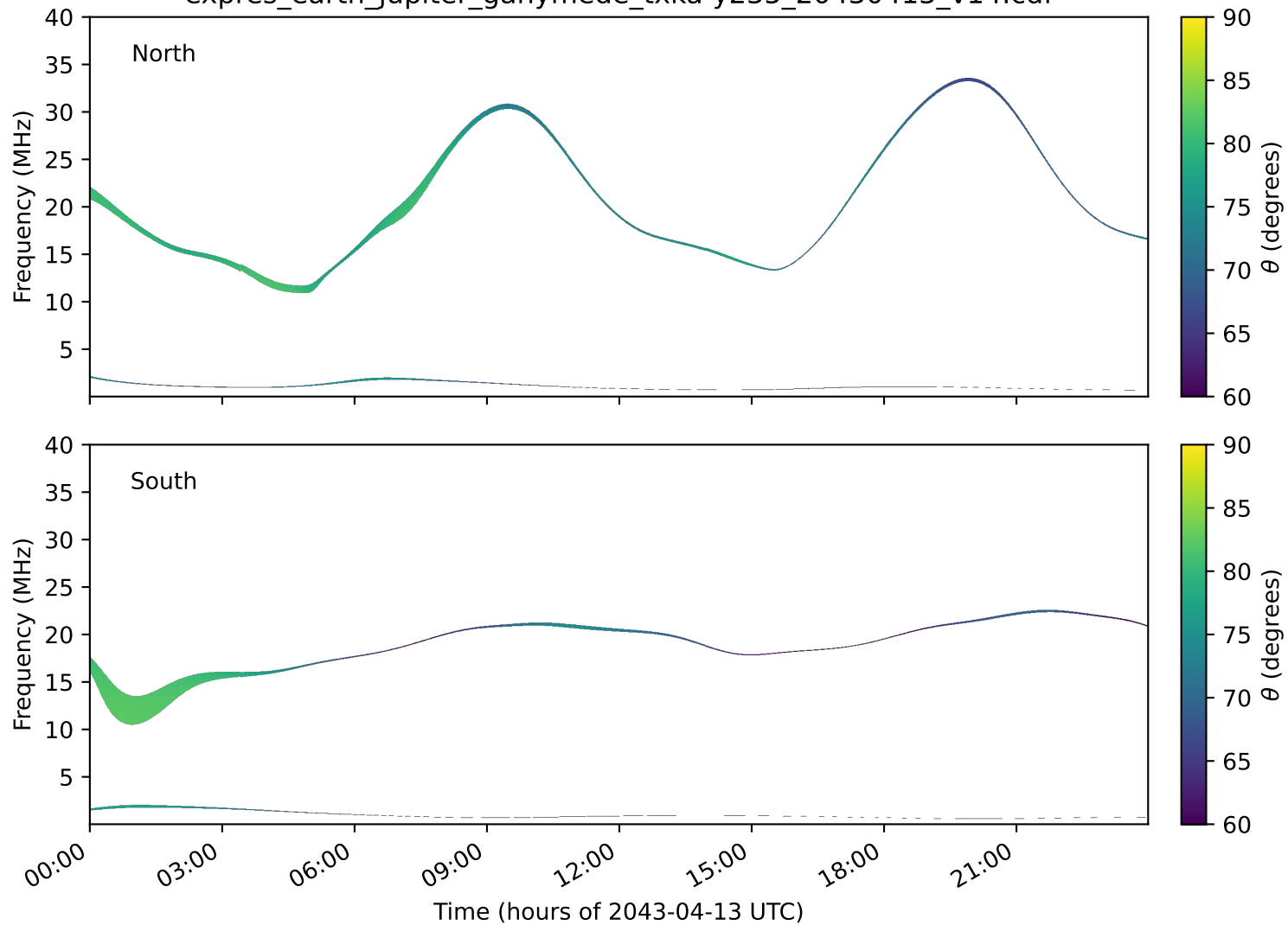
expres_earth_jupiter_ganymede_txka-y235_20430413_v14.cdf
