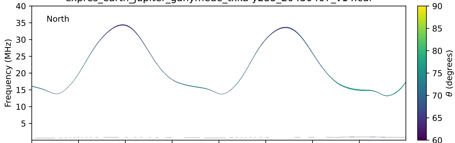
expres_earth_jupiter_ganymede_txka-y235_20430407_v14.cdf
