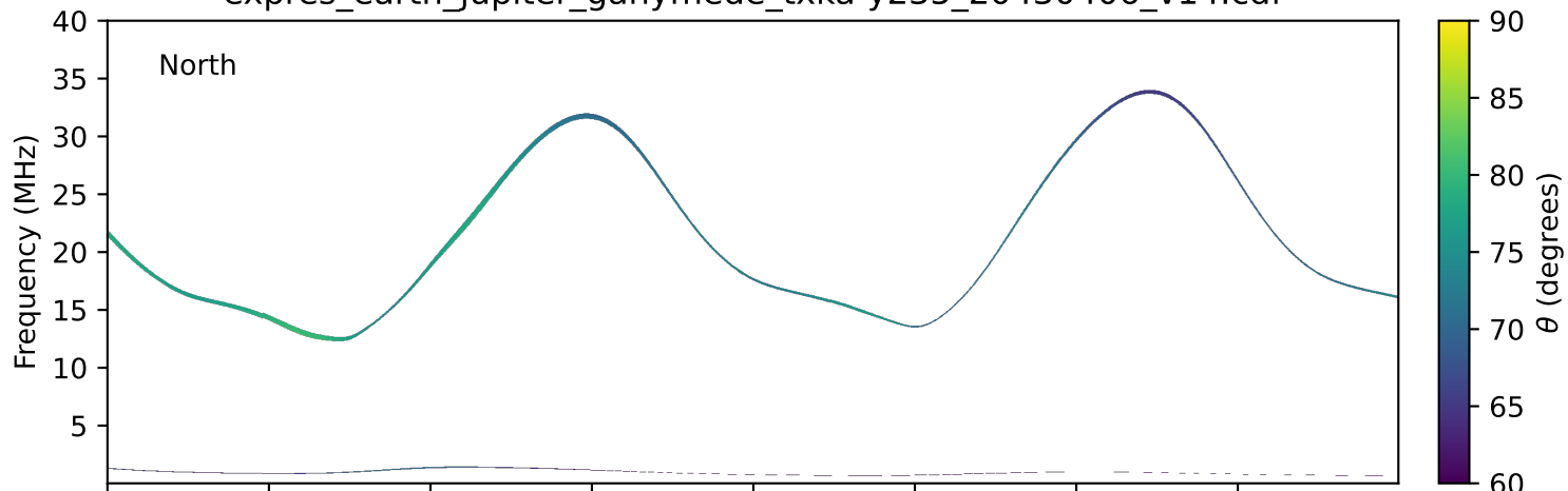
expres_earth_jupiter_ganymede_txka-y235_20430406_v14.cdf
